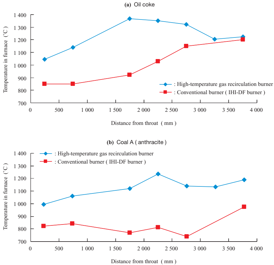
Fig. 7 Temperature distribution in furnace measured via observation windows
