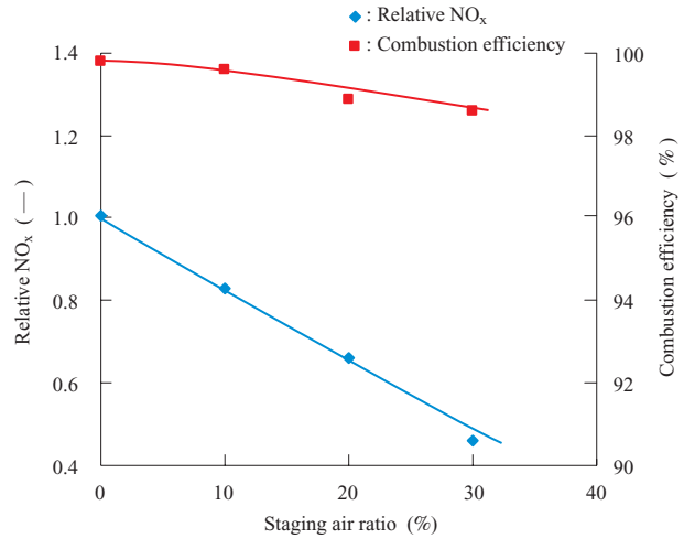
Fig. 9 Combustion characteristics ( Oil coke )
