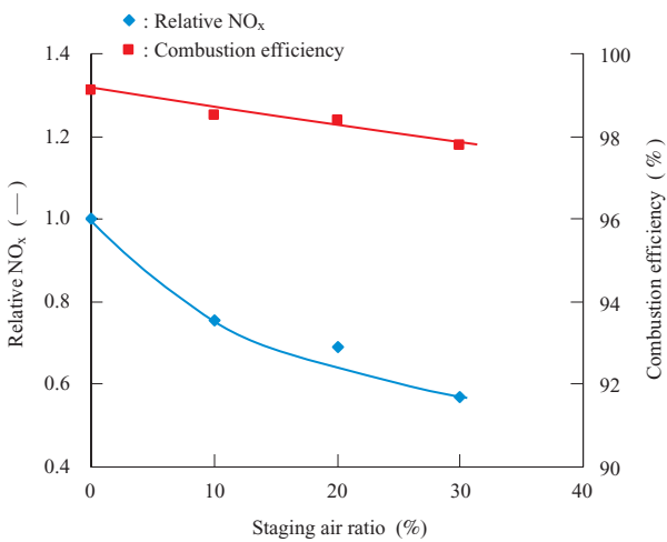
Fig. 8 Combustion characteristics ( Coal B )
