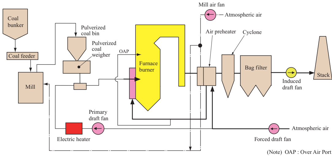
Fig. 2 Schematic diagram of combustion test facility
