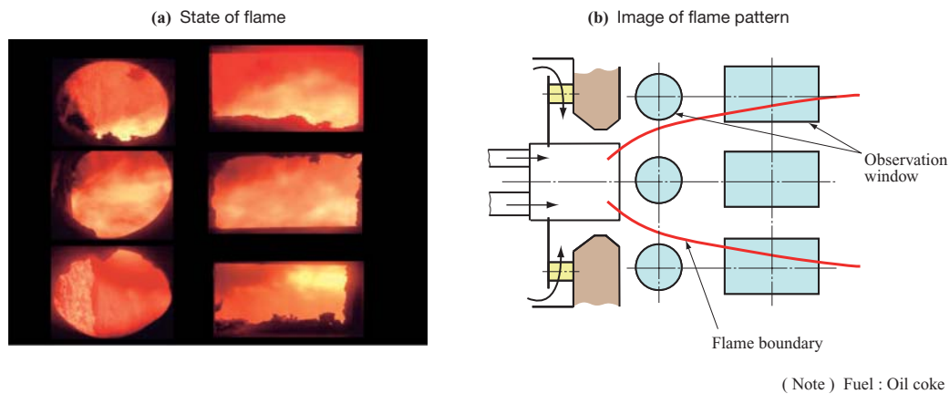
Fig. 5 Flame state using high-temperature gas recirculation burner
