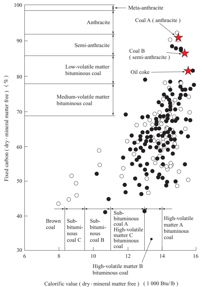
Fig. 3 ASTM classification of coal grade
