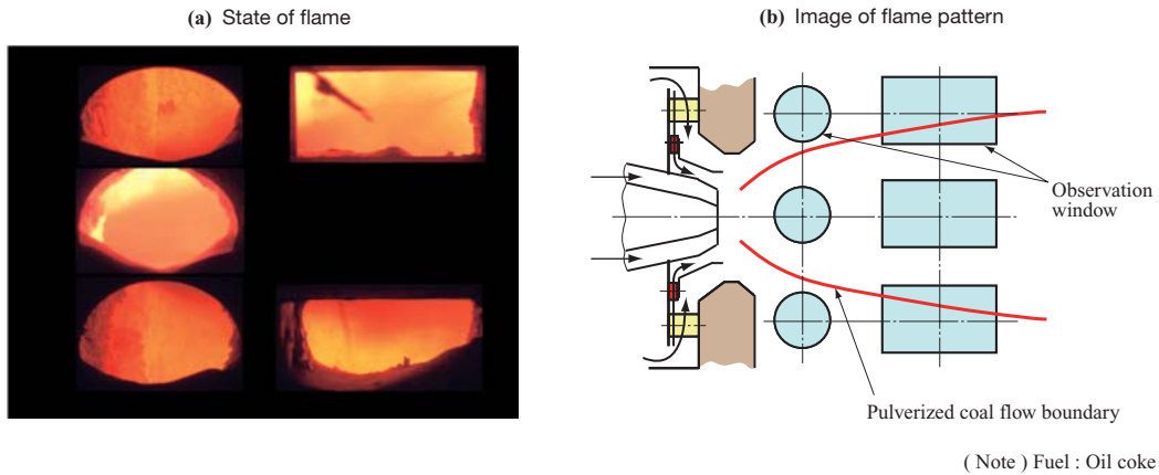
Fig. 4 Flame state using IHI-DF burner
