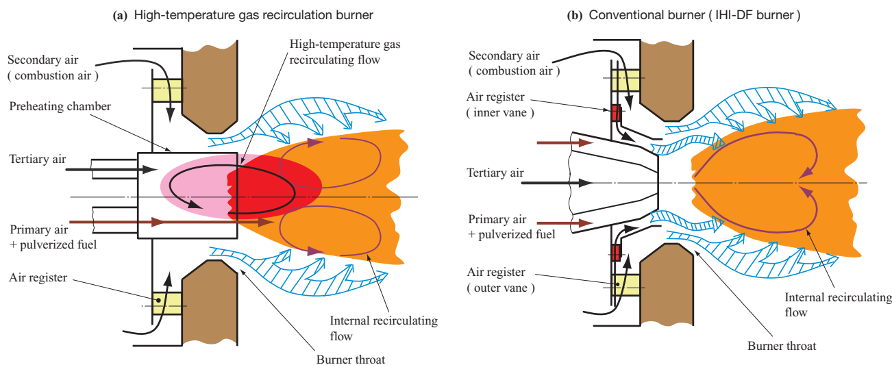
Fig. 1 Concept of high-temperature gas recirculation burner and IHI-DF burner
