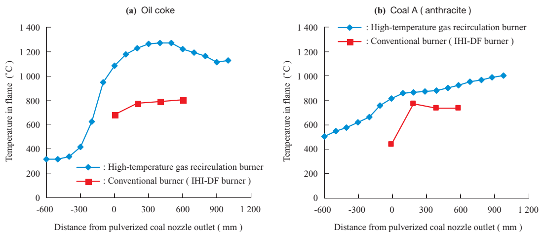
Fig. 6 Flame temperature distribution along the burner centerline
